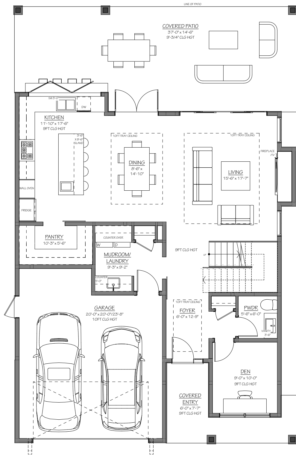
MAIN FLOOR
