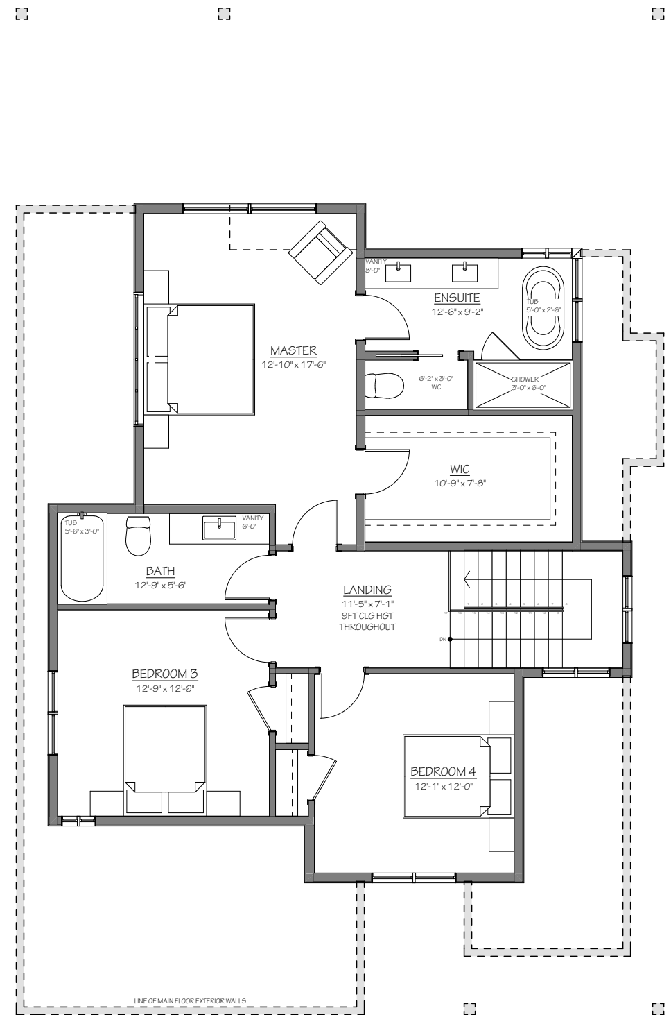
UPPER FLOOR
