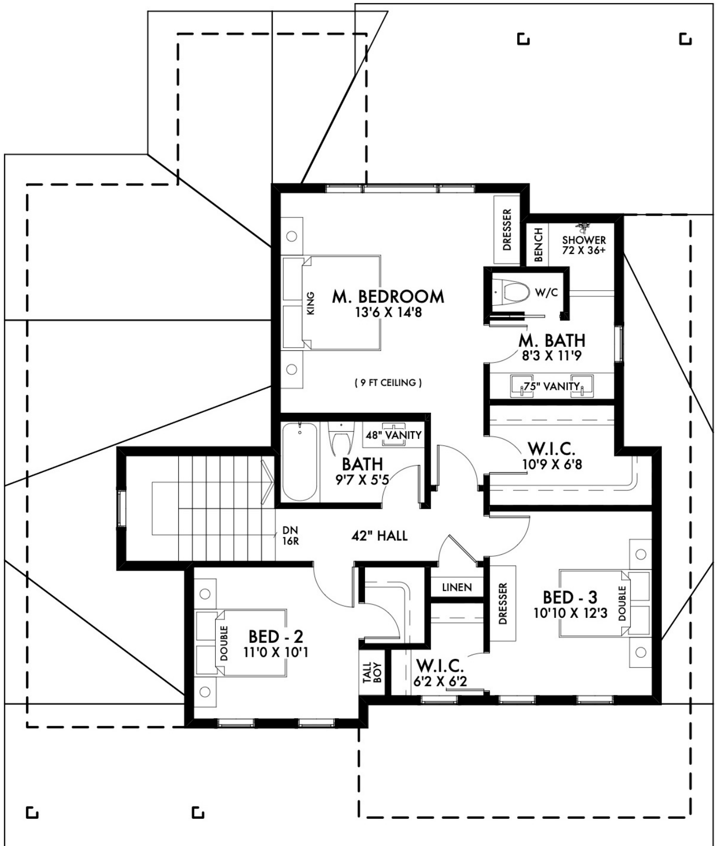
UPPER FLOOR FLOOR AREA: 903 SQ. FT
